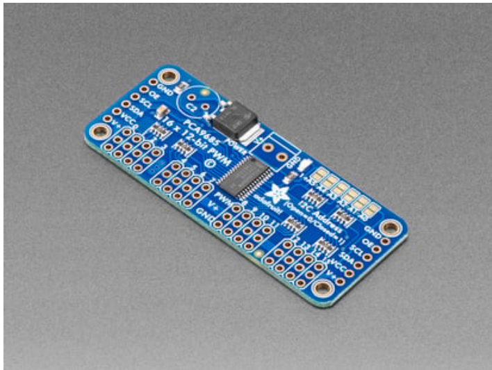
Adafruit 16-Channel 12-bit PWM/Servo Driver - I2C interface - PCA9685 - PCA9685
